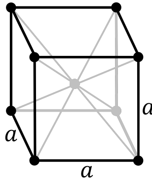
body centered cubic
