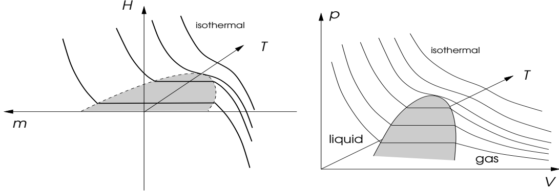
Fig. 5.6: Left panel: phase diagram of ferromagnetic Ising model in (H, m, T) ; right panel: phase diagram of the liquid-gas transition in (p, V, T) . In both cases the shaded region represents a coexistence region.
