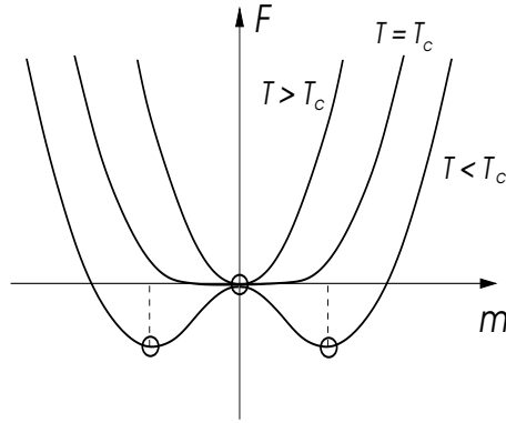
Fig. 5.2: Landau free energy: T > T_c : 2 nd -order term is positive and minimum of F at m = 0 ; T = T_c , 2 nd vanishes and free energy minimum at m = 0 becomes very shallow; T < T_c : 2 nd -order term is negative and minimum of F is at finite value of m , bounded by the 4 th -order term.
